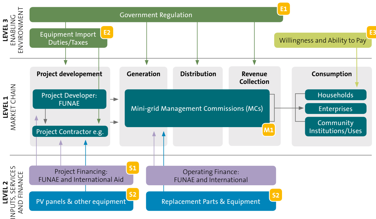
Figure 17 FUNAE Mini-Grid Market System Model
