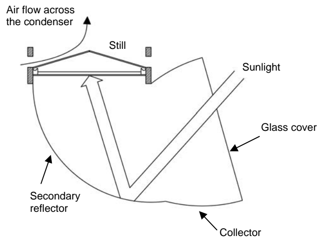
Figure 3: An inverted absorber solar still. Illustration: Neil Noble / Practical Action.
