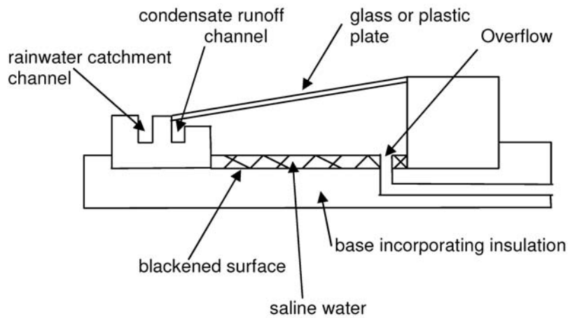
Figure 1: Schematic of a single-basin still. Illustration: Otto Ruskulis for Practical Action.
